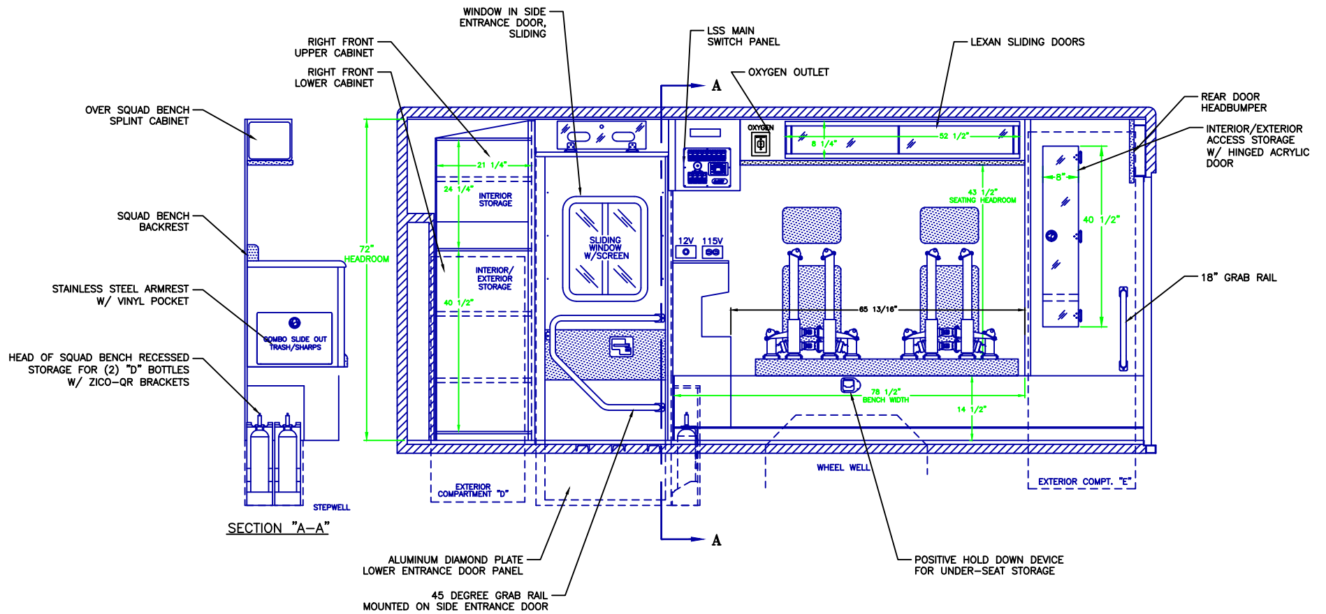
CURBSIDE VIEW
