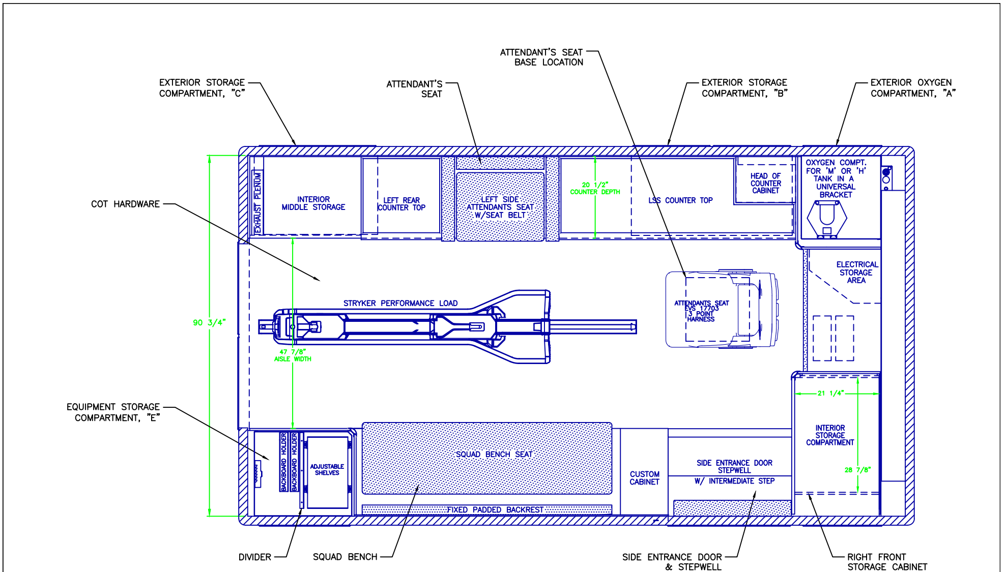
FLOOR PLAN
